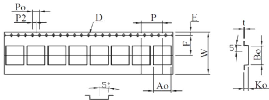
Figure 5-2: Tape Dimensions
