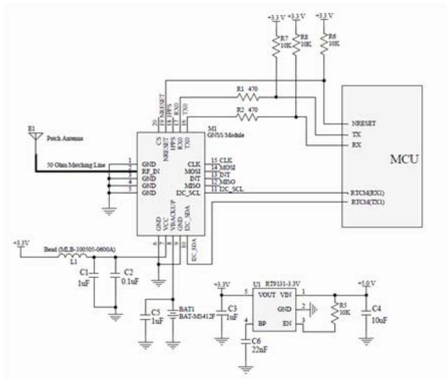
Figure 4-1: UART + RTCM
